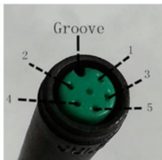
connection wire end to display end
